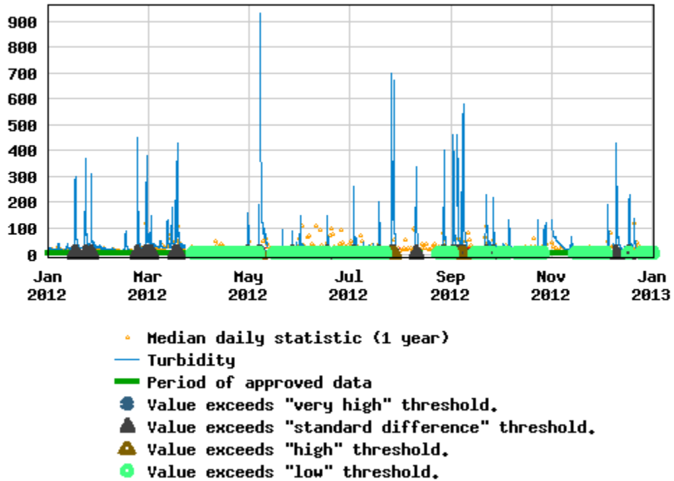
USGS 04208800 Cuyahoga River at Independence OH
