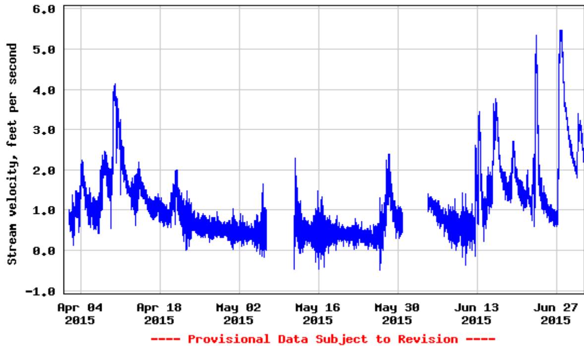
USGS 04208504 Cuyahoga River near Newburgh Heights OH
