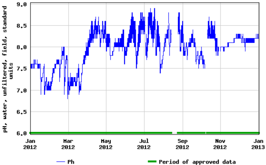
USGS 04208000 Cuyahoga River at Independence OH
