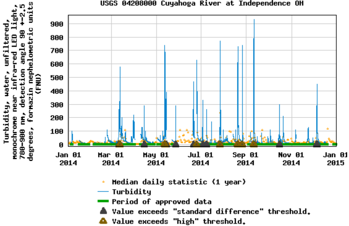
USGS 04208000 Cuyahoga River at Independence OH
